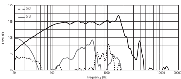
2 nd and 3 rd harmonic distortion levels have been raised 20dB. Measurements made at 10% of rated power.
